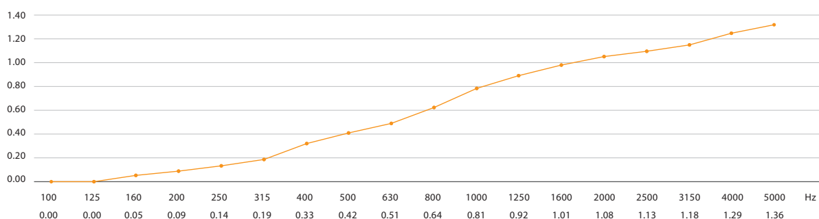
m 2 /Sab Equivalent Absorption Area
